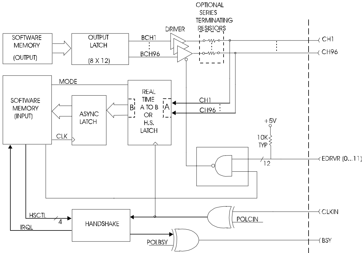
Figure 1-1, 1260-14 Block Diagram
